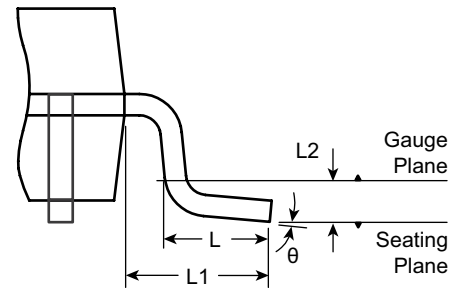
View B
