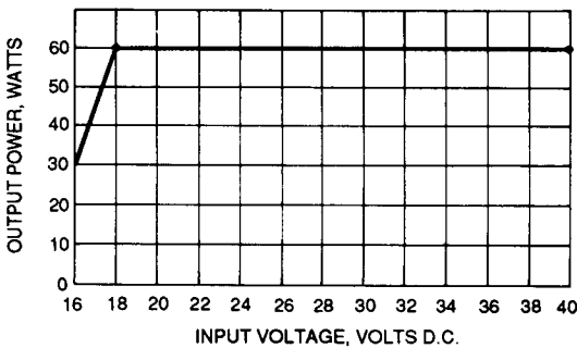
FIGURE 4. OUTPUT POWER VS. INPUT VOLTAGE
