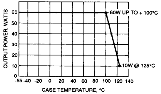
FIGURE 2. OUTPUT POWER VS. CASE TEMPERATURE
