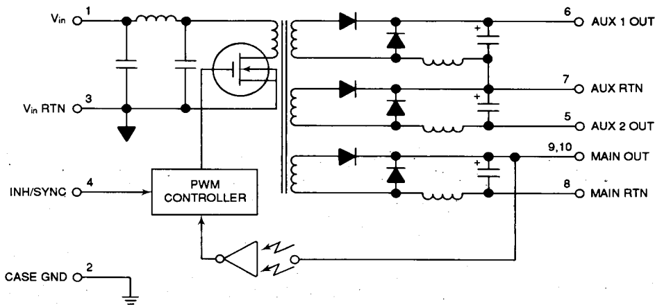
FIGURE 1. PWR-82400 SERIES BLOCK DIAGRAM
