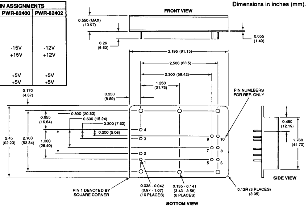
FIGURE 6. MECHANICAL OUTLINE
