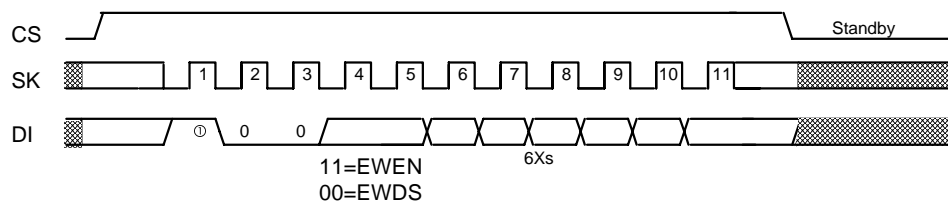
Figure 10 EWEN/EWDS Timing (S-29Z330A)
