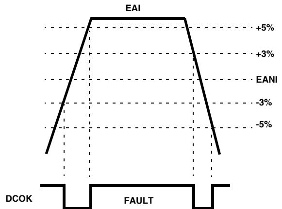
FIGURE 11. UNDERVOLTAGE-OVERVOLTAGE WINDOW
