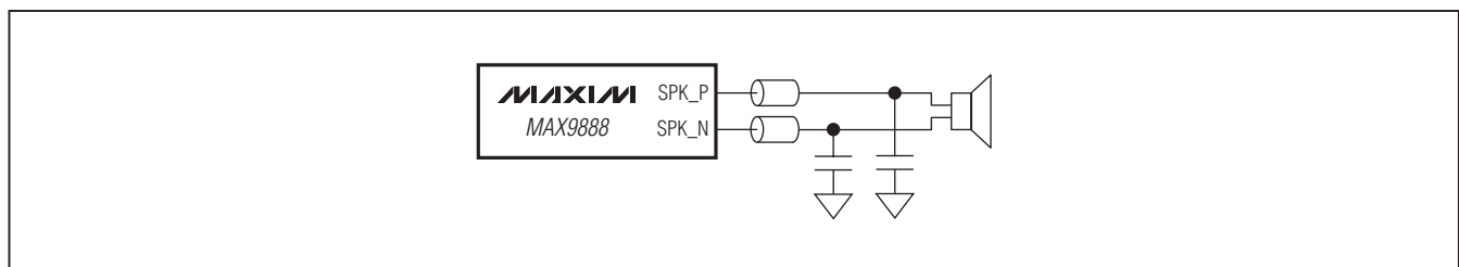
Figure 41. Optional Class D Ferrite Bead Filter
