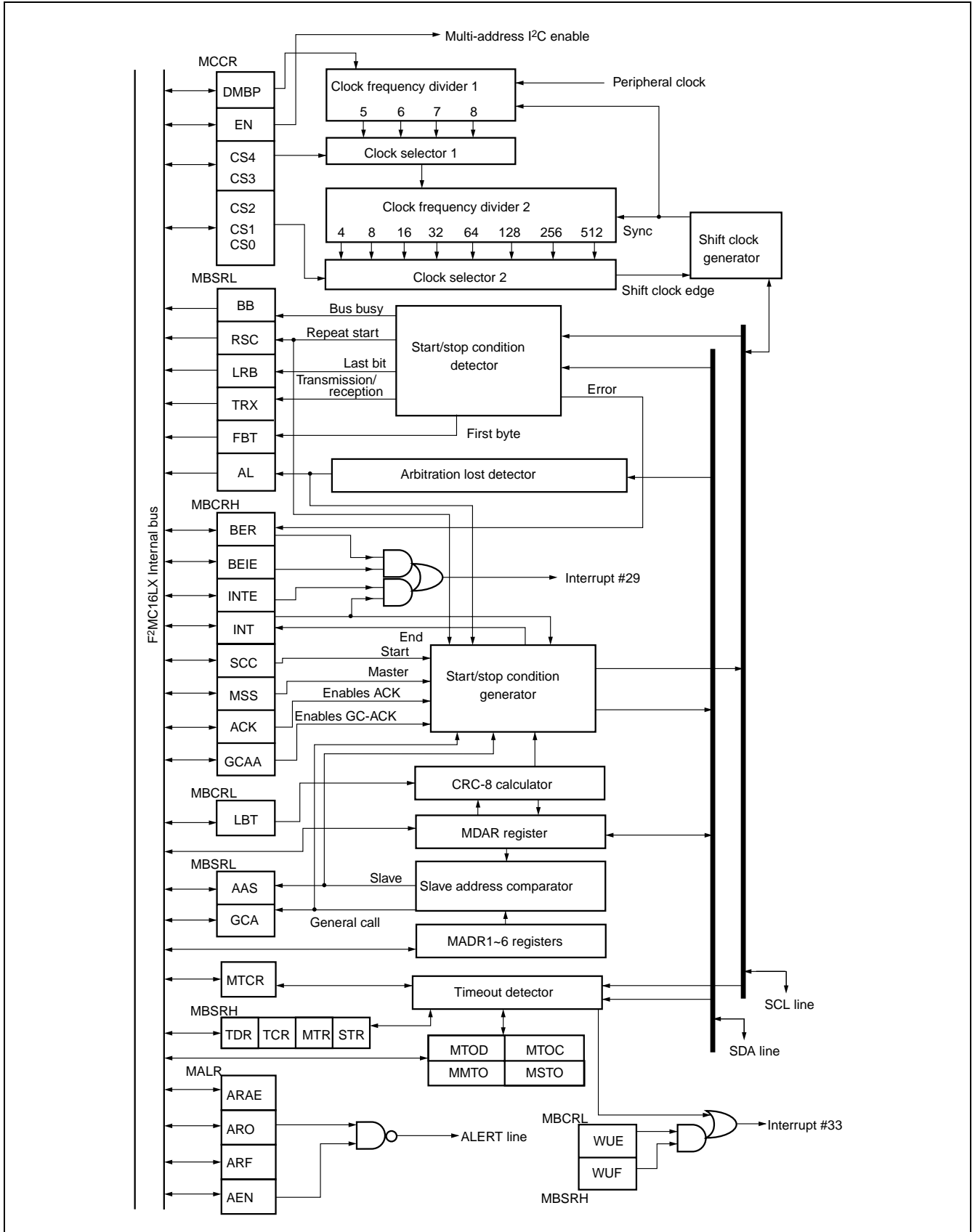
(2) Block diagram of MI 2 C
