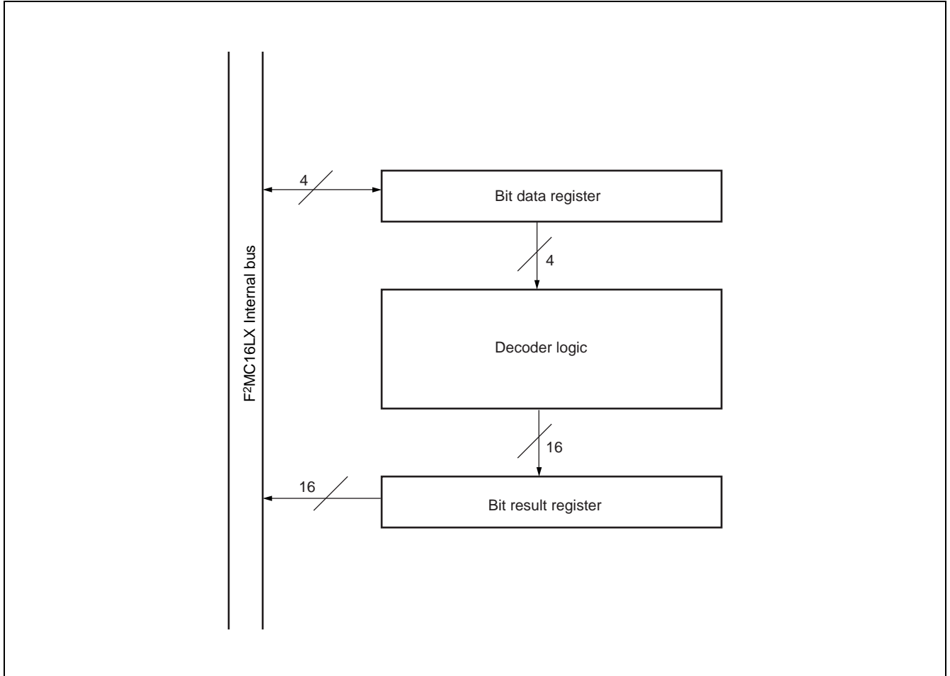
(2) Block diagram of bit decoder
