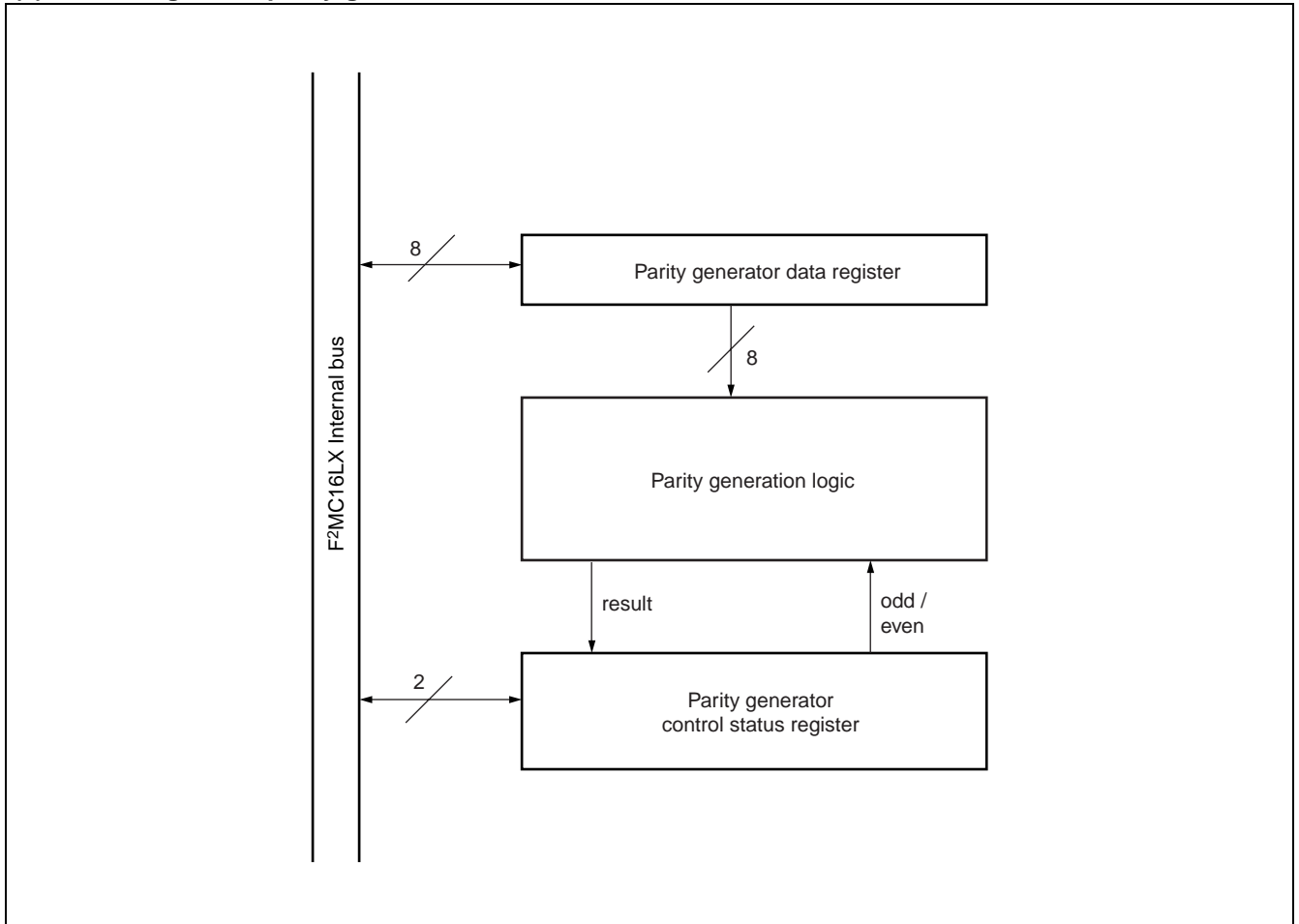
(2) Block diagram of parity generator
