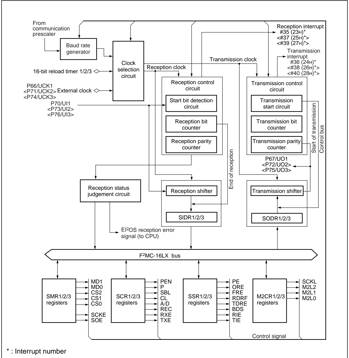
(2) Block diagram of UART
