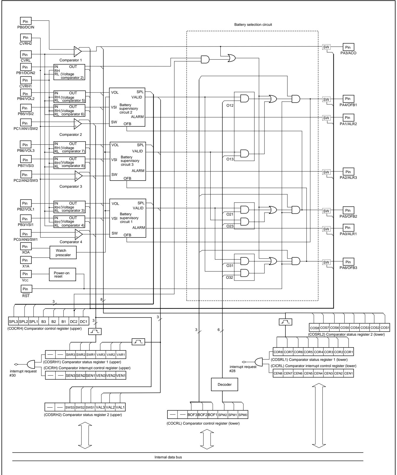
(2) Block diagram of comparator
