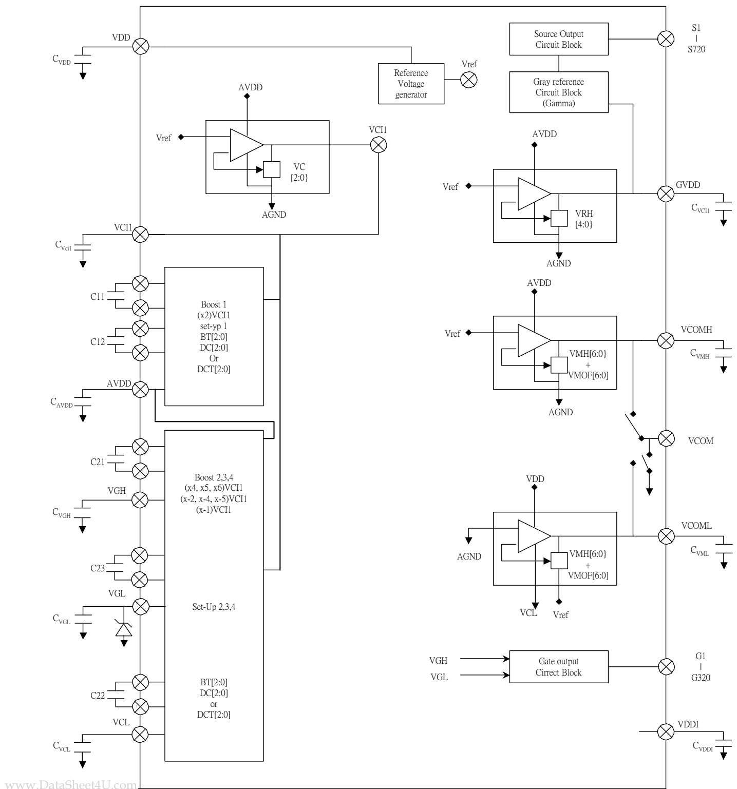
Fig. 12.2.1 Power Booster Structure (1)
