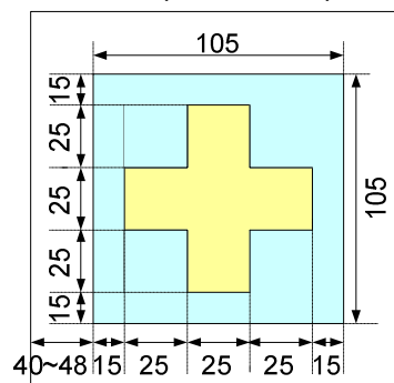
Alignment mark R ("+" type)
