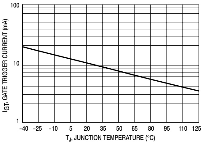
Figure 6. Typical Gate Trigger Current versus Junction Temperature
