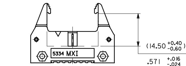
90897-2*** STRAIN RELIEF VERSION
