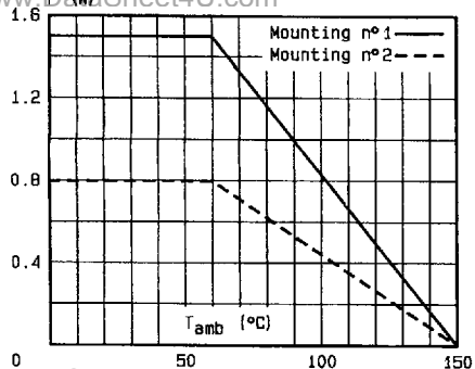
Fig.1 - Power dissipation versus ambient temperature.
