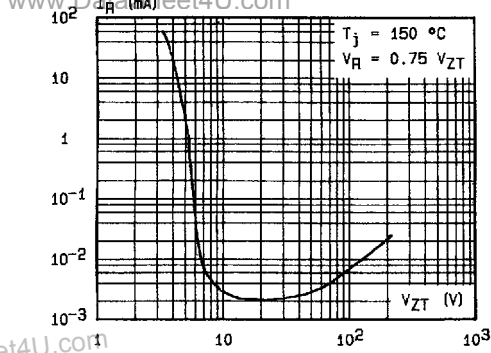
Fig. 6 - Reverse current versus regulation voltage (typical values).
