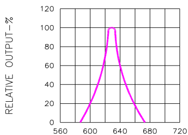
Fig.2 SPECTRAL RESPONSE
