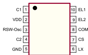
10-Lead MSOP (MG)
