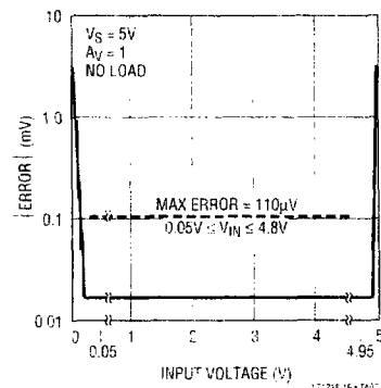
Voltage Follower Input to Output Error
