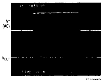
Figure 7a. LT1218 Power Supply Rejection Test
