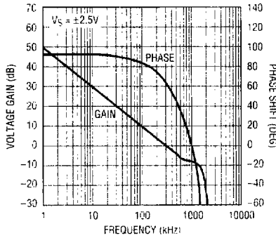
LT1218 Gain and Phase Shift vs Frequency
