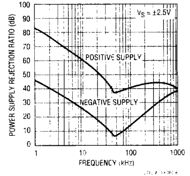
LT1219 Power Supply Rejection Ratio vs Frequency
