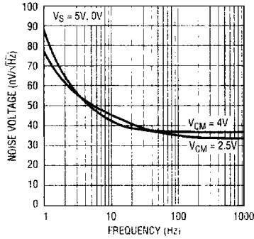
Noise Voltage Spectrum
