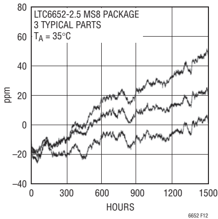
Figure 12. Long-Term Drift
