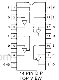
SPXXHC126 Quad 3-State Buffers with Active High Enables
