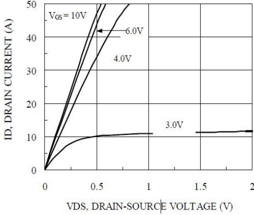
Figure 1. On-Region Characteristics
