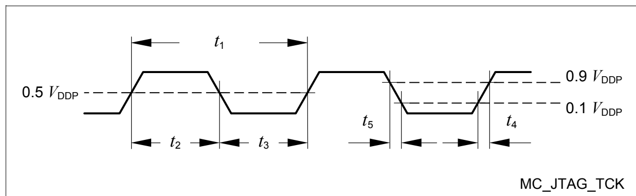
Figure 22 Test Clock Timing (TCK)
