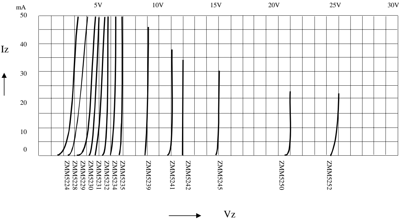
FIG.1- BREAKDOWN CHARACTERISTICS
