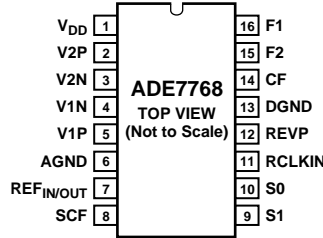
Figure 3. Pin Configuration
