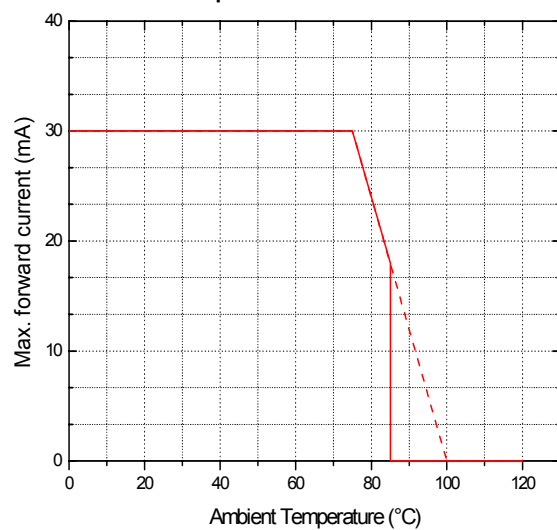
Ambient Temperature vs. maximal forward current
