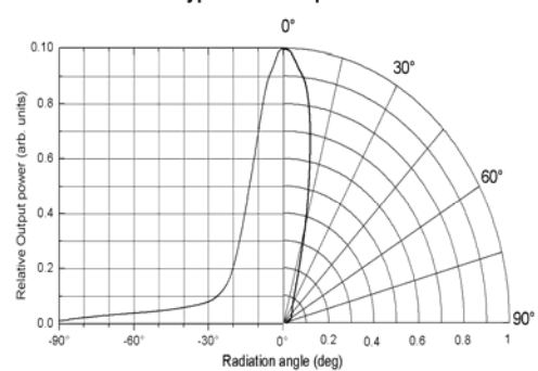
Typical radiant pattern
