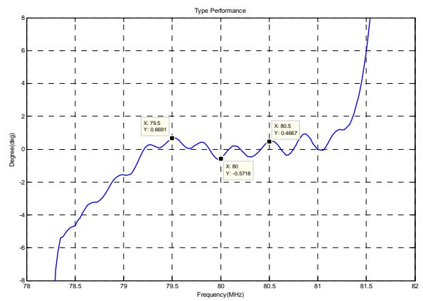
Phase Linearity(f0±0.5MHz)
