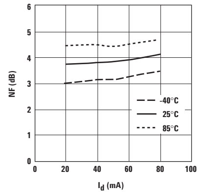
Figure 11. NF vs. I_d and Temperature at 900 MHz.
