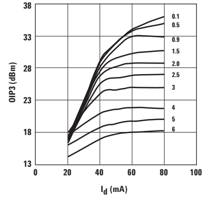
Figure 14. OIP_3 vs. I_d and Frequency (GHz).
