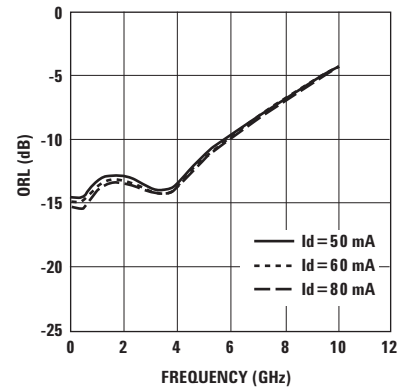
Figure 17. Output Return Loss vs. I_d and Frequency.
