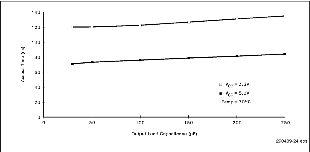
Figure 21. Access Time ( t_{ACC} ) vs. Output Loading
