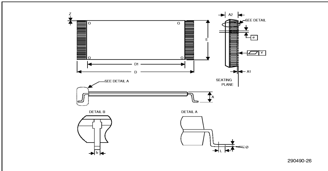
Figure 24. Mechanical Specifications of the Dual Die 56-Lead TSOP Type I Package
