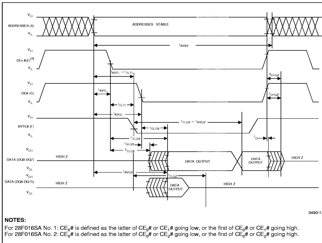
Figure 12. BYTE# Timing Waveforms
