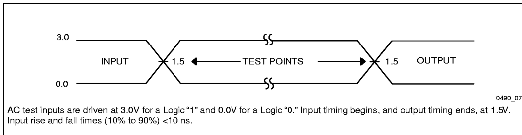
Figure 7. Transient Input/Output Reference Waveform ( V_{CC} = 3.3V ) and High Speed Reference Waveform (2) ( V_{CC} = 5.0V \pm 5\% )
