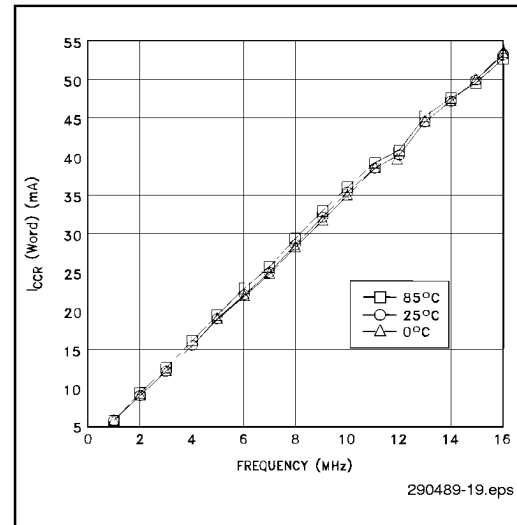
Figure 19. I_{CC} vs. Frequency ( V_{CC} = 3.6V ) for x8 or x16 Operation
