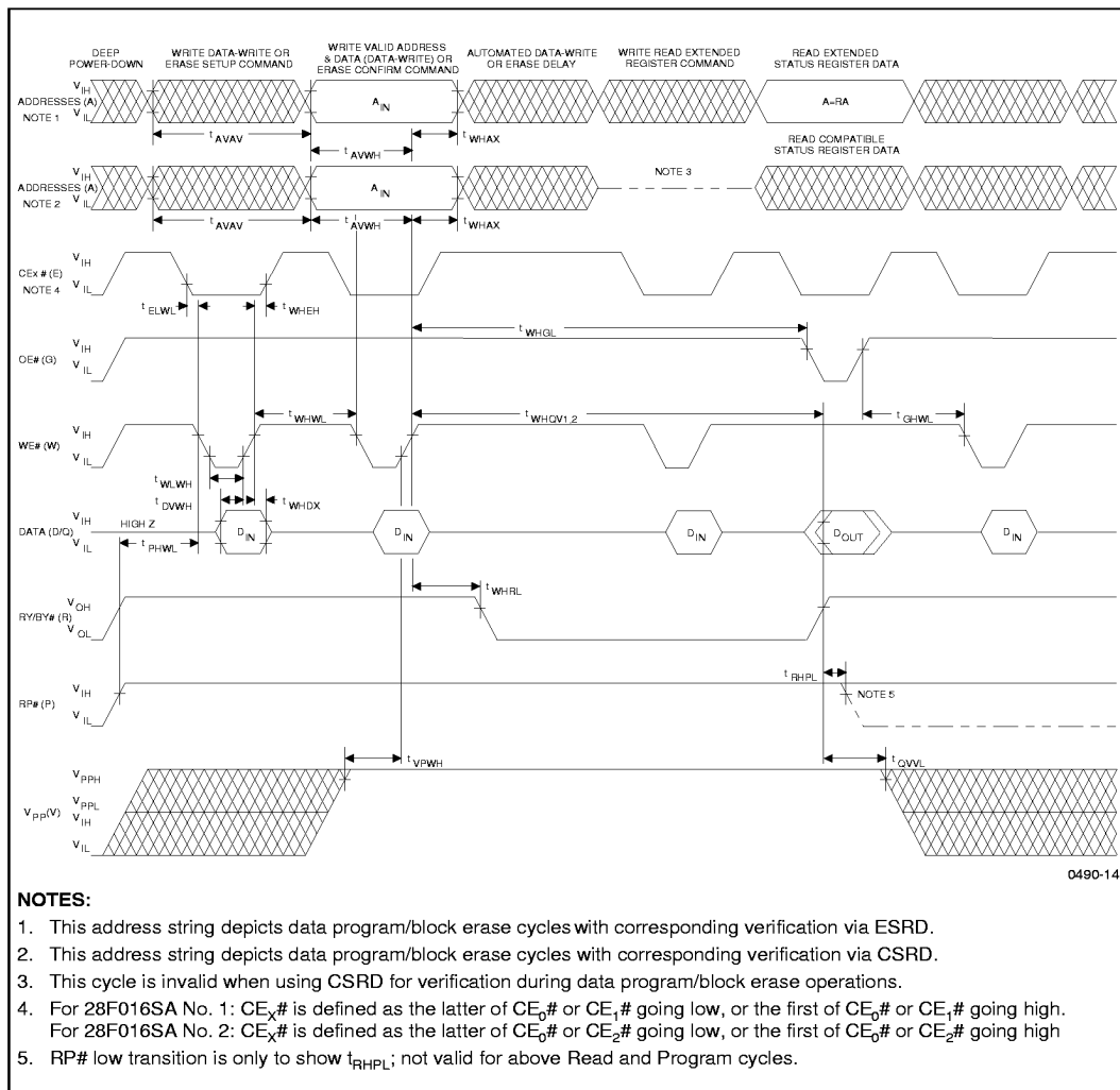
Figure 14. AC Waveforms for Command Write Operations
