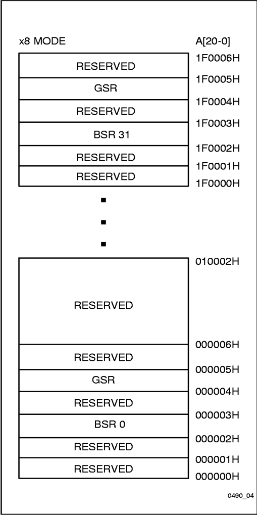
Figure 4. Extended Status Register Memory Map (Byte-Wide Mode)
