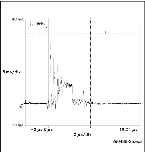
Figure 22. I_{PP} during Word Write Operation
