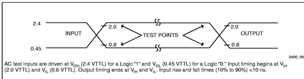
Figure 6. Transient Input/Output Reference Waveform ( V_{CC} = 5.0V ) for Standard Test Configuration (1)
