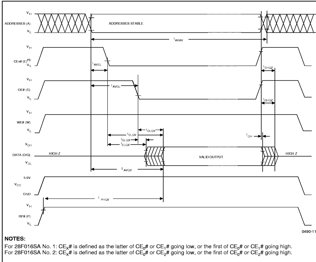
Figure 11. Read Timing Waveforms
