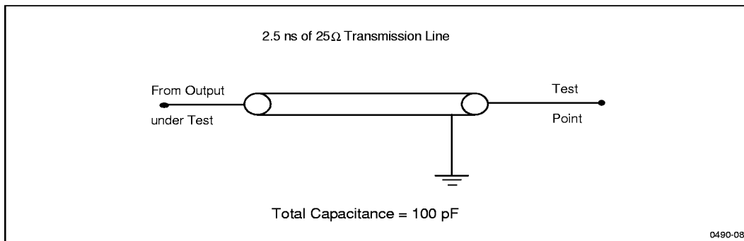
Figure 8. Transient Equivalent Testing Load Circuit ( V_{CC} = 5.0V \pm 10\% )
