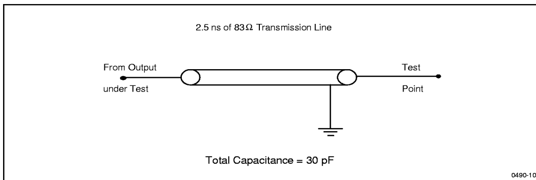
Figure 10. High Speed Transient Equivalent Testing Load Circuit ( V_{CC} = 5.0V \pm 5\% )
