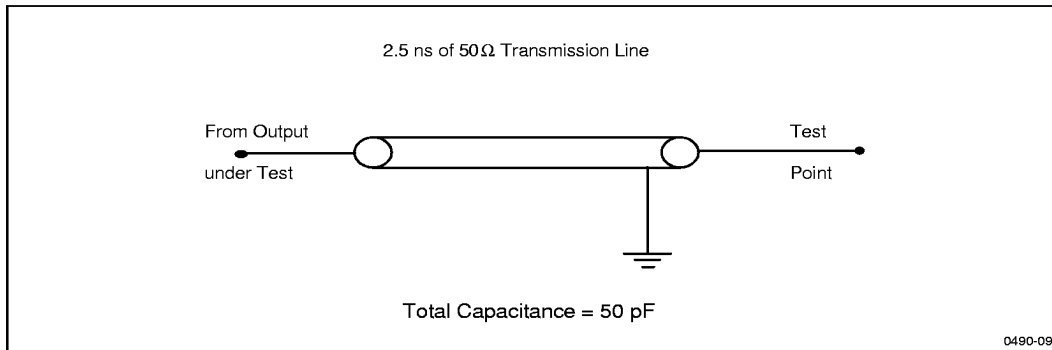
Figure 9. Transient Equivalent Testing Load Circuit ( V_{CC} = 3.3V \pm 0.3V )
