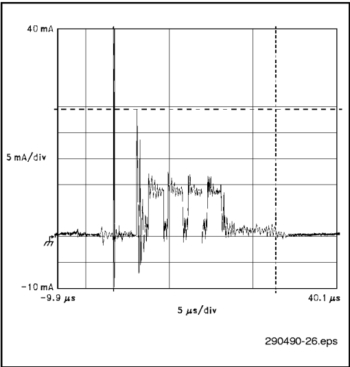
Figure 23. I_{PP} during Page Buffer Write Operation
