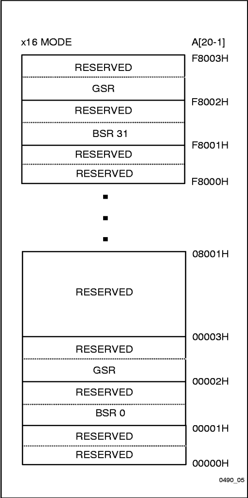
Figure 5. Extended Status Register Memory Map (Word-Wide Mode)
