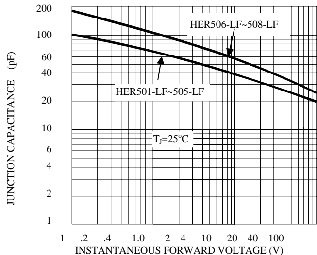
FIG. 6-TYPICAL JUNCTION CAPACITANCE
