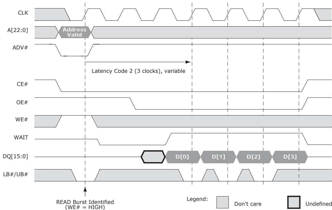
Figure 29.4 Burst Mode Read (4-word burst)
