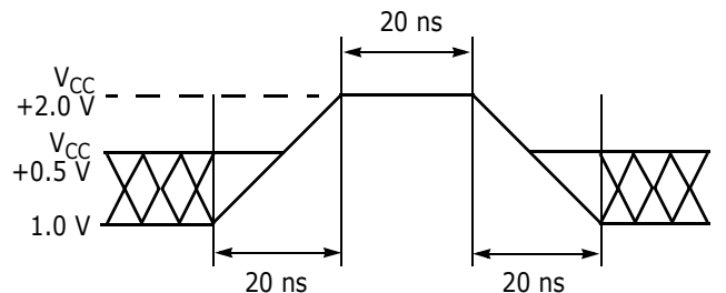
Figure 22.7 Maximum Positive Overshoot Waveform
