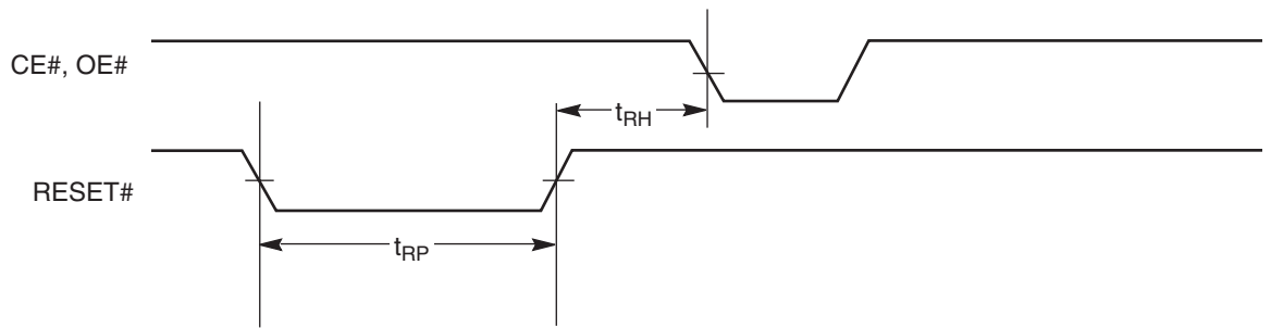
Reset Timings
