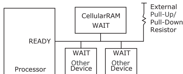
Figure 29.6 Wired or Wait Configuration
