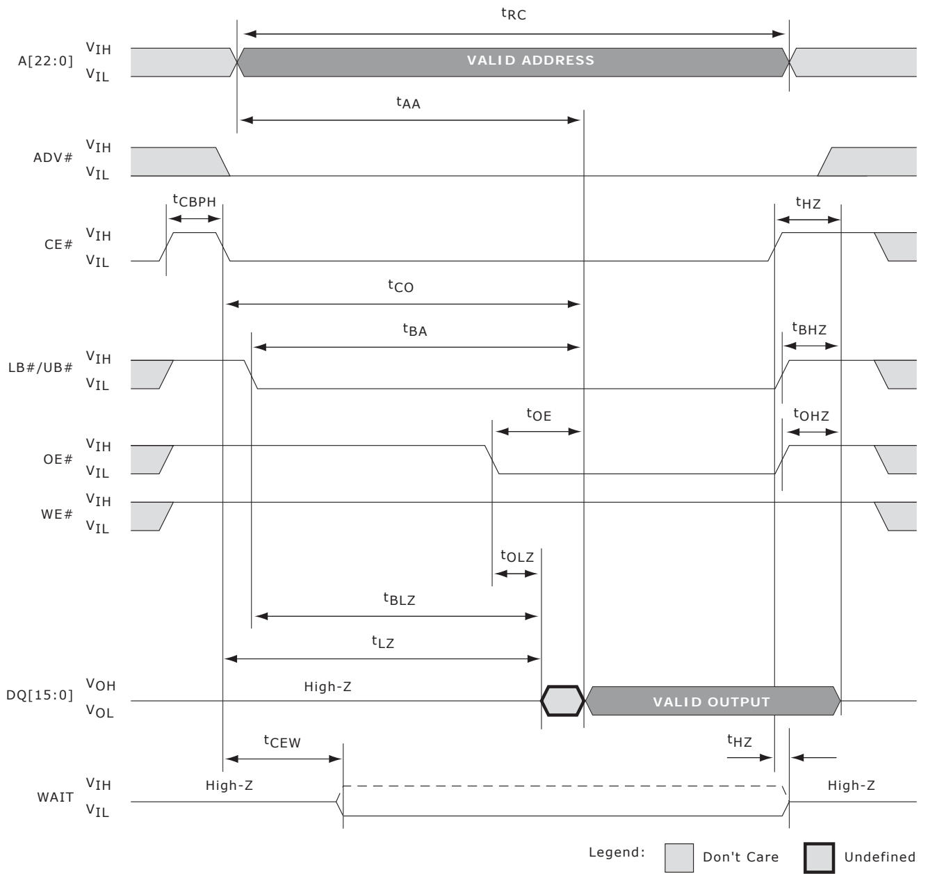
Figure 34.4 Asynchronous Read
