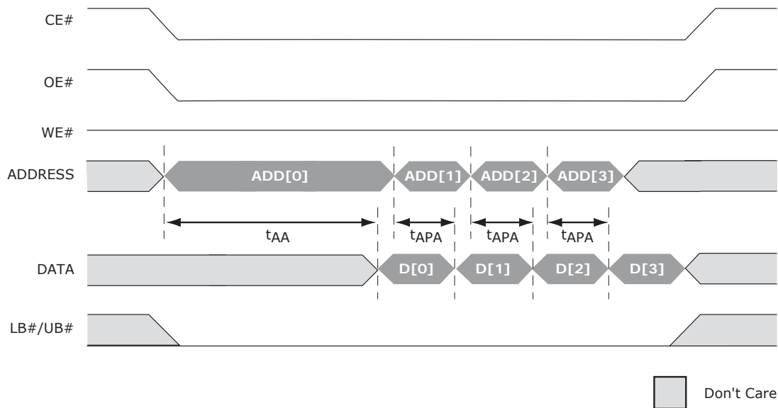
Figure 29.3 Page Mode Read Operation (ADV# Low)
