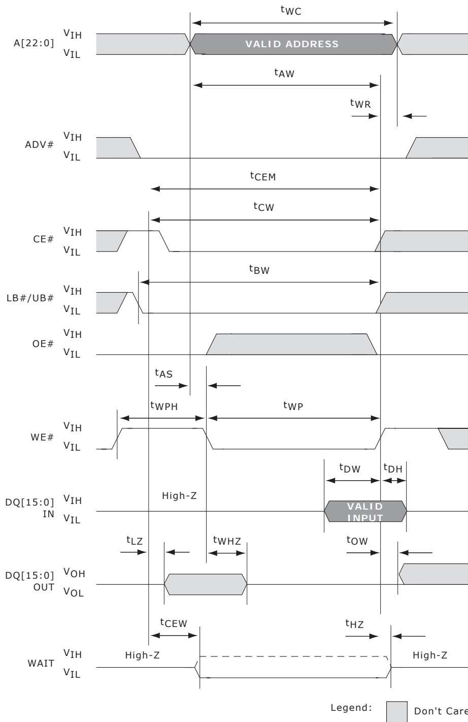
Figure 34.13 WE#-Controlled Asynchronous Write
