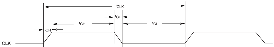
Figure 25.2 CLK Characterization
