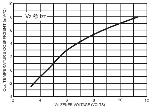
FIG.3- ZENER VOLTAGE - TO 12 VOLTAGES
