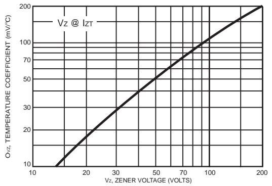
FIG.4- ZENER VOLTAGE - 14 TO 200 VOLTAGES
