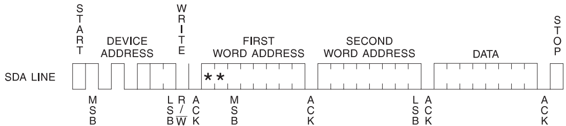
Figure 8. Byte Write
