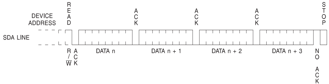
Figure 12. Sequential Read
