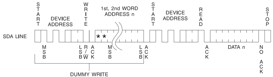
Figure 11. Random Read
