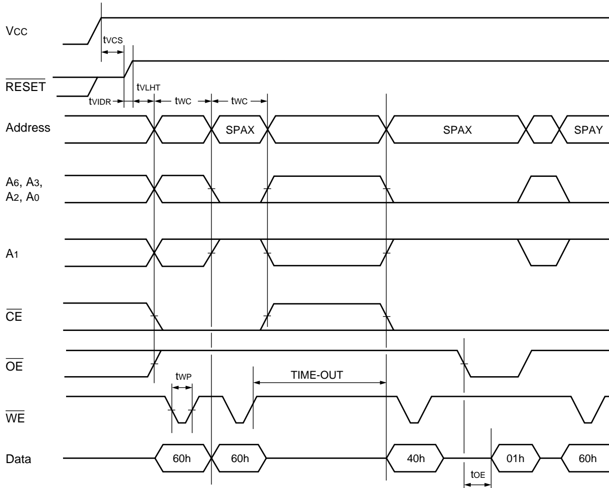
(17) Extended Sector Group Protection Timing Diagram
