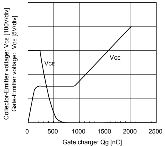
Dynamic Gate Charge (typ.) V CC = 300V, I C = 600A, T j = 25°C
