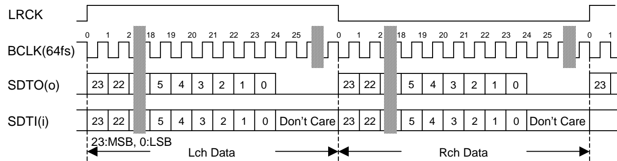
Figure 25. Mode 2 Timing
