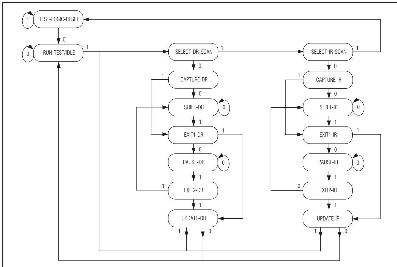
www.DataSheet4U.com Figure 11. Tap Controller State Diagram
