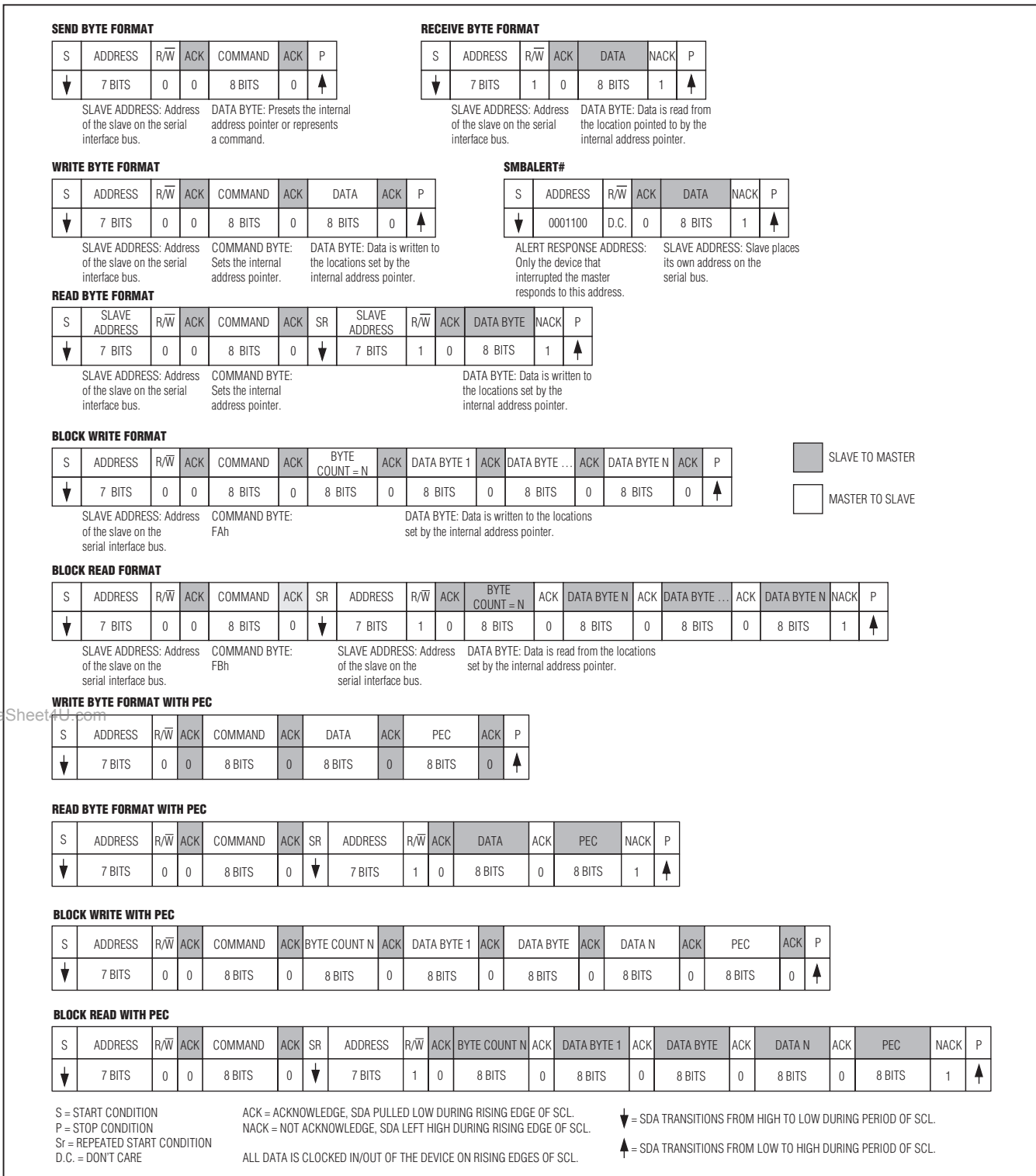
Figure 9. SMBus Protocols
