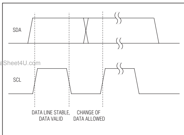
Figure 6. Bit Transfer
