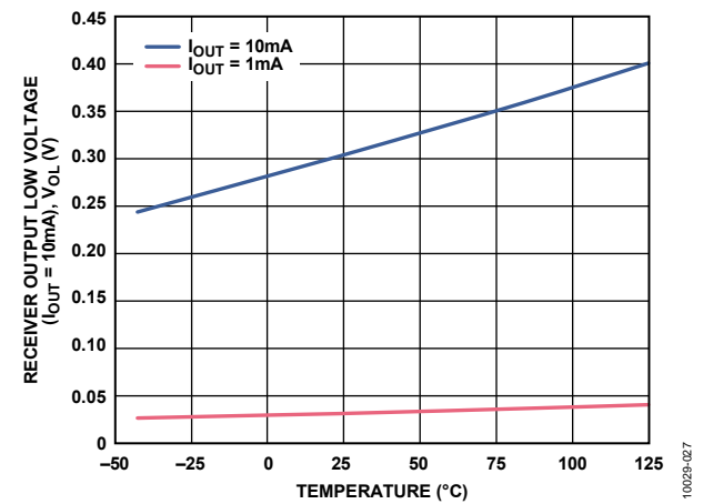
Figure 20. Receiver Output Low Voltage vs. Temperature
