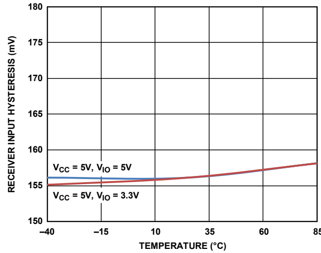
Figure 8. Receiver Input Hysteresis vs. Temperature
