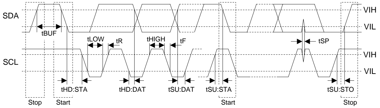
Figure 8. I²C Bus Mode Timing
