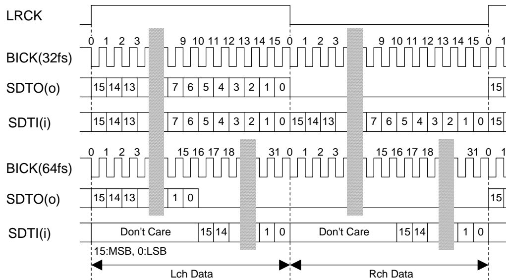
Figure 14. Mode 0 Timing
