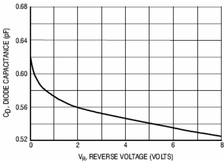
Figure 3. Capacitance
