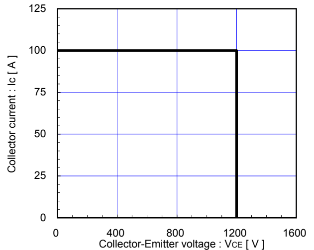
Reverse bias safe operating area (max.) +V_{GE}=15V, -V_{GE} \le 15V, R_G \ge 22\Omega, T_j \le 125^\circ C
