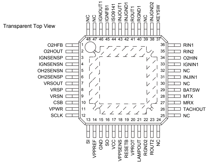
Figure 3. 33813 Pin Connections
