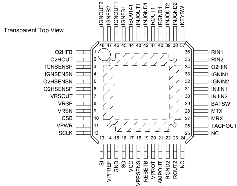
Figure 3. 33814 Pin Connections
