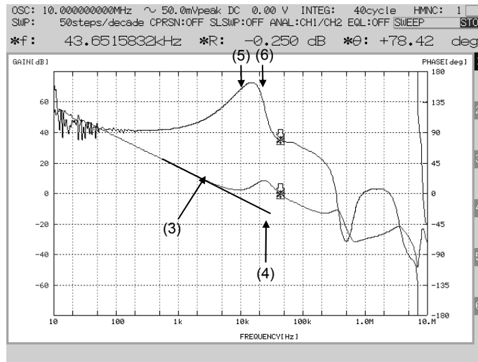
Fig.31 Example of DC/DC converter frequency property (Measured with FRA5097 by NF Corporation)
