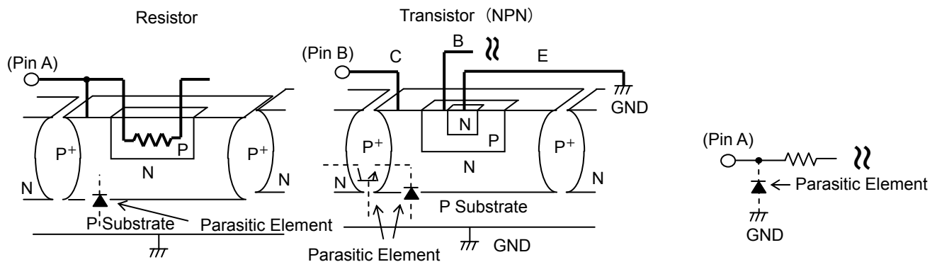
Fig.32 Example of simple structure of Bipolar IC
