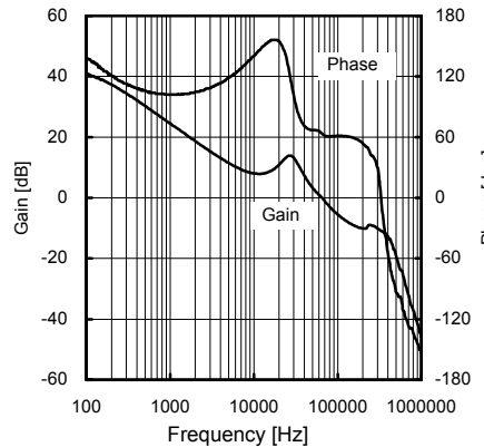
Fig.27 Frequency response 8 (VCC=10V, Io=500mA)
