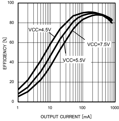
Fig.18 Power conversion efficiency (VOUT = 3.3 V)
