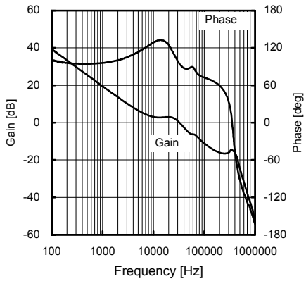
Fig.21 Frequency response 2 (VCC=6.0V, Io=250mA)
