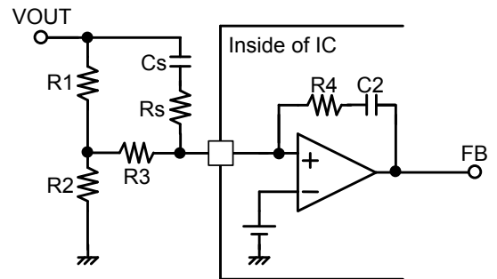
Fig.30 Example of phase compensation setting
