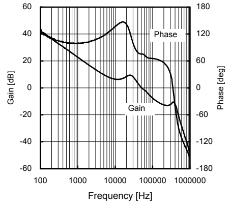
Fig.22 Frequency response 3 (VCC=8.4V, Io=250mA)
