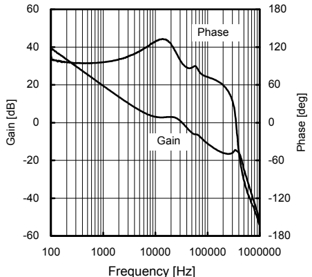
Fig.25 Frequency response 6 (VCC=6.0V, Io=500mA)
