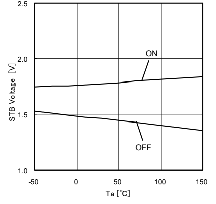
Fig.14. STB threshold temperature property
