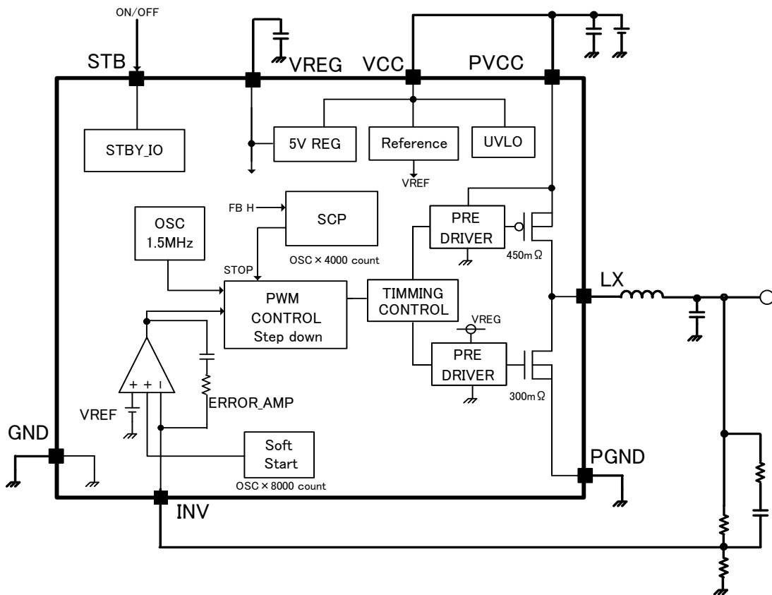
Fig.2 Block diagram
