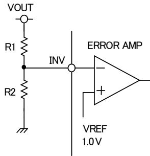
Fig.29 Setting of voltage feedback resistance
