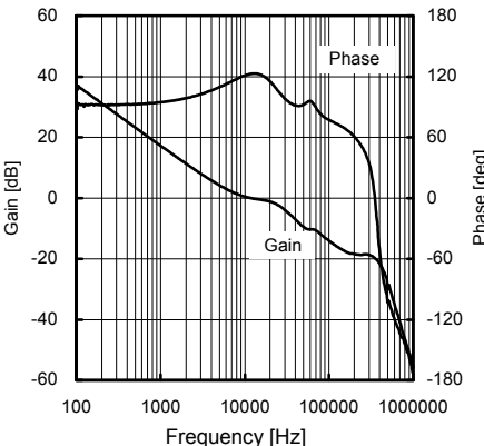
Fig.24 Frequency response 5 (VCC=4.5V, Io=500mA)
