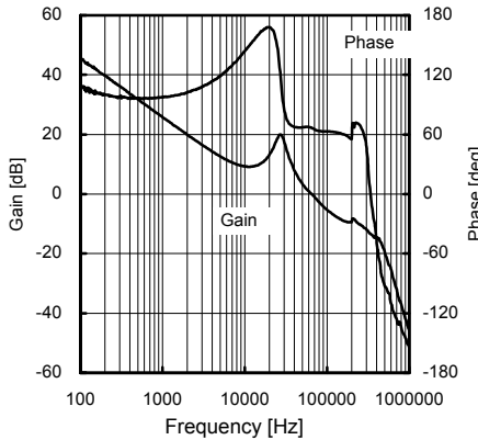
Fig.23 Frequency response 4 (VCC=10V, Io=250mA)
