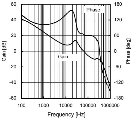
Fig.20 Frequency response 1 (VCC=4.5V, Io=250mA)
