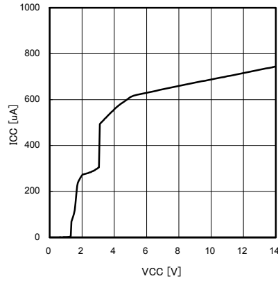
Fig.16. Circuit current voltage property
