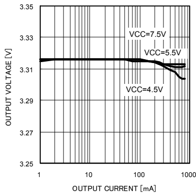
Fig.19 Load regulation (VOUT = 3.3 V)
