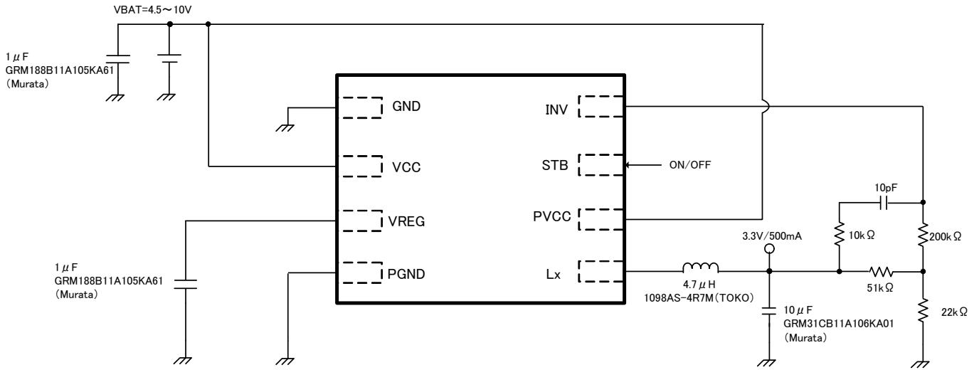
Fig.17 Reference application diagram
