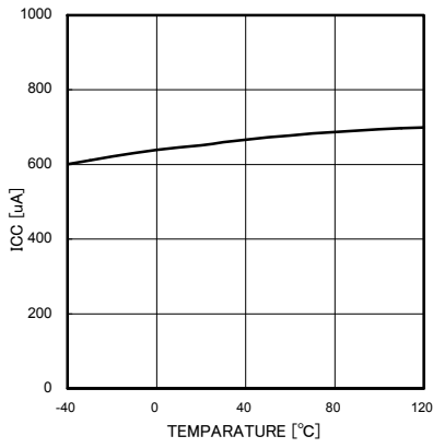
Fig.15. Circuit current temperature property
