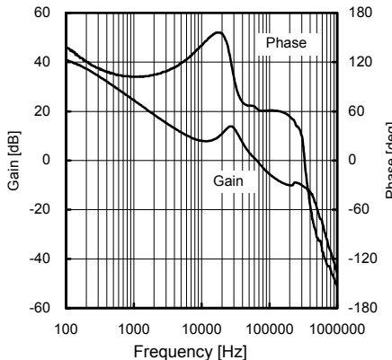
Fig.26 Frequency response 7 (VCC=8.4V, Io=500mA)
