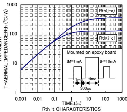
Rth-t CHARACTERISTICS
