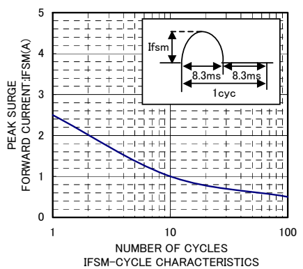
IFSM-CYCLE CHARACTERISTICS
