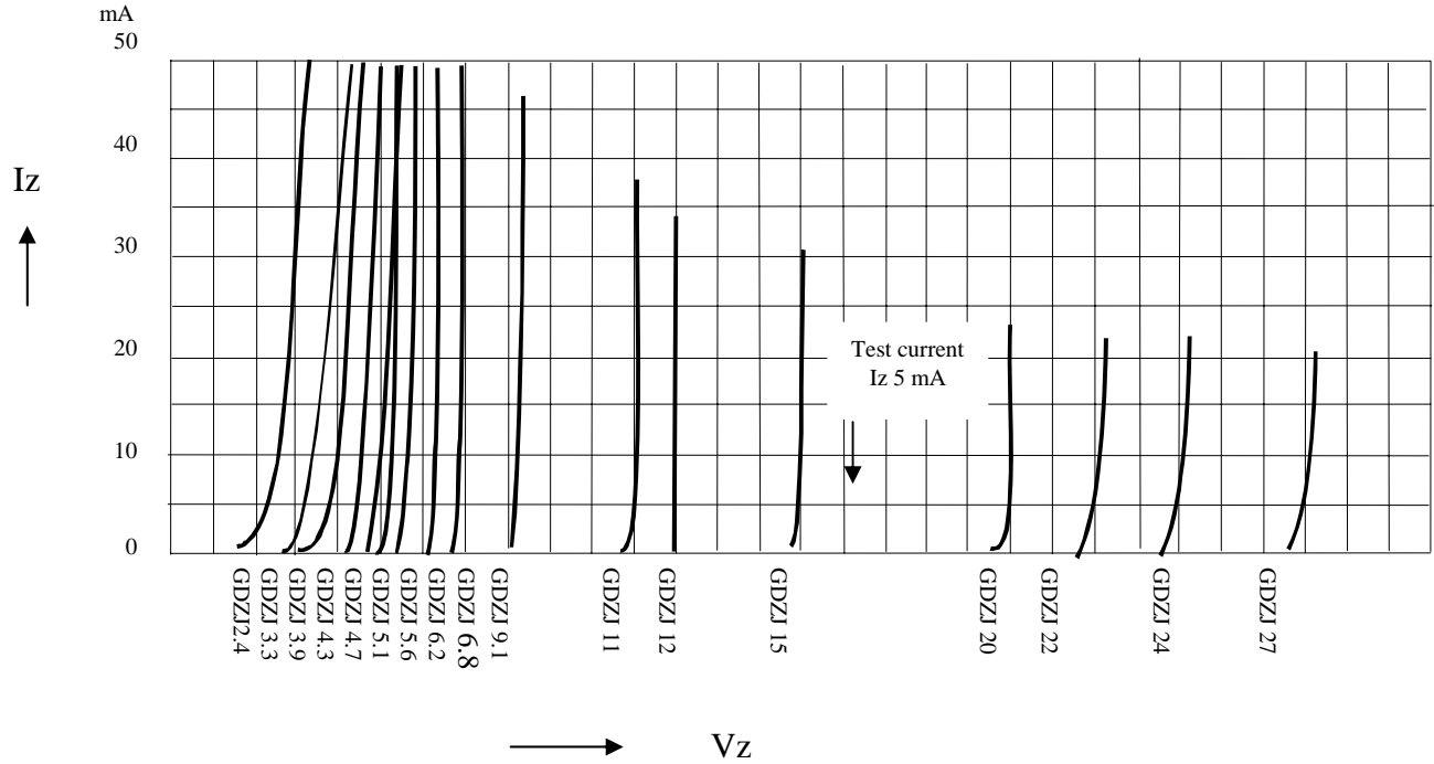
FIG.1- BREAKDOWN CHARACTERISTICS
