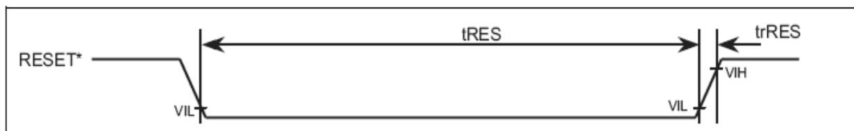
Figure 100 Reset Operation
