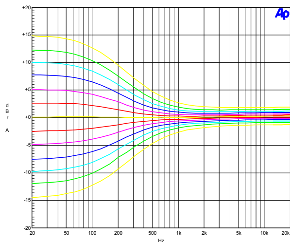
Figure 18 Base Response vs. Frequency VDD=5V, RL=8ohm, BTL
