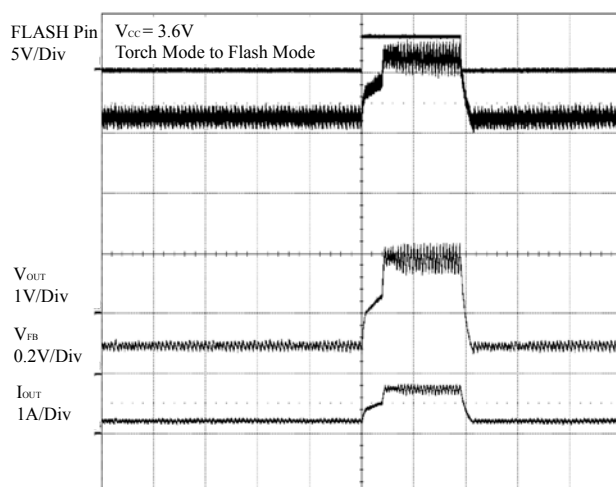
Figure 6 Torch Mode to Flash Mode
