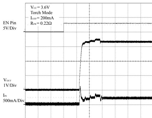
Figure 4 EN On (Torch Mode)
