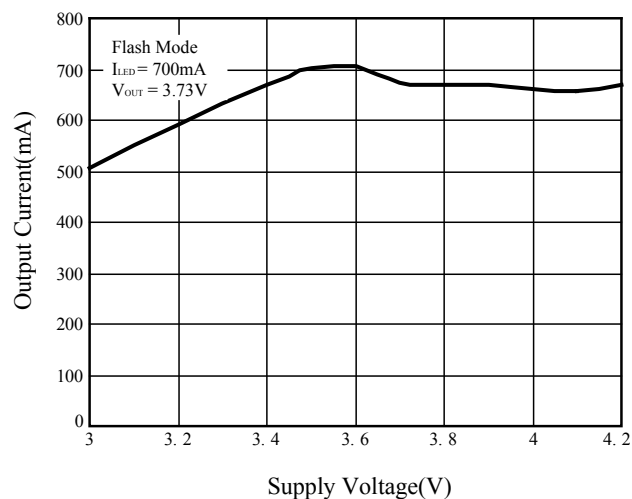
Figure 3 Supply Voltage vs. Output Current (Flash Mode)
