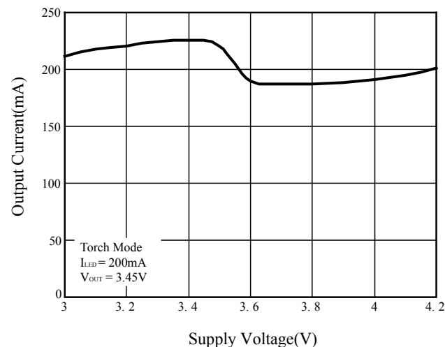
Figure 2 Supply Voltage vs. Output Current (Torch Mode)
