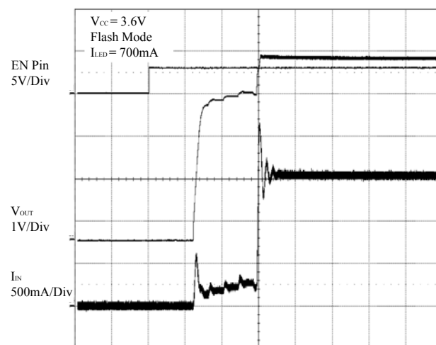
Figure 5 EN On (Flash Mode)
