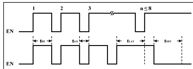
Figure 8 EN pin timing
