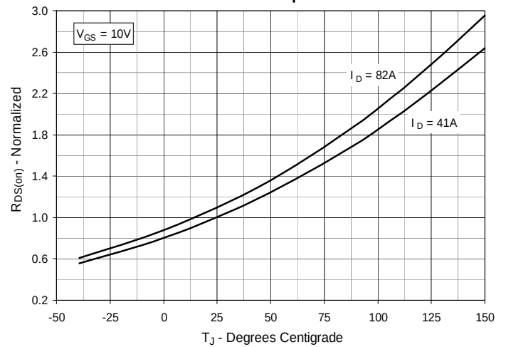
Fig. 4. R_{DS(on)} Normalized to I_D = 41\text{A} Value vs. Junction Temperature
