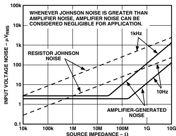
Figure 15. Total Noise vs. Source Impedance
