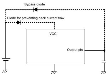
Fig. 32 Bypass diode
