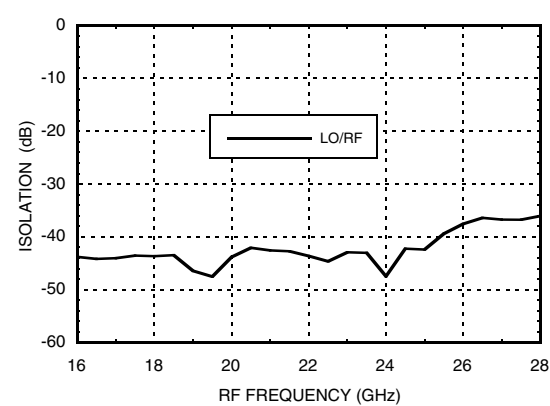
LO/RF Isolation
