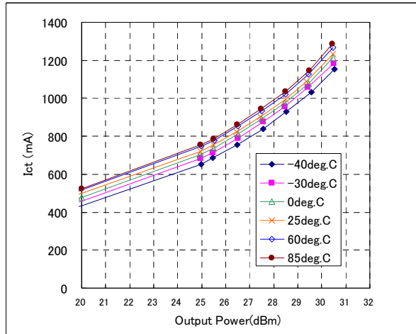
Operating Current vs. Output Power
