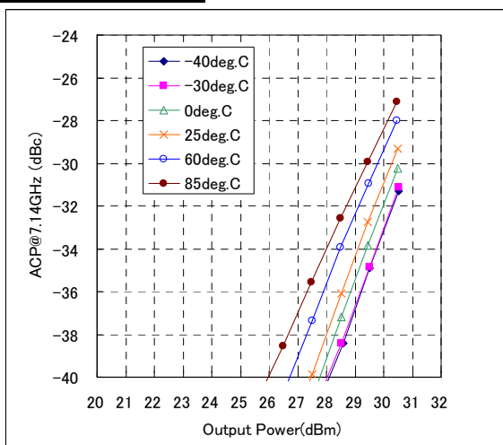
ACP Characteristics
