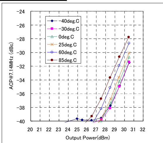
ACP Characteristics
