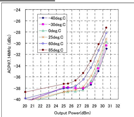
ACP Characteristics
