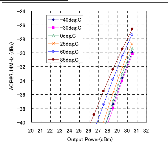
ACP Characteristics
