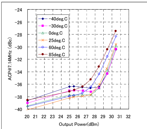
ACP Characteristics
