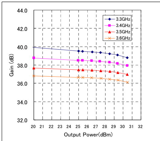
Gain vs. Output Power
