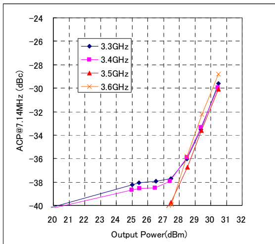
ACP Characteristics
