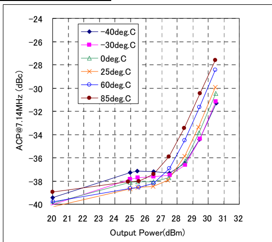
ACP Characteristics
