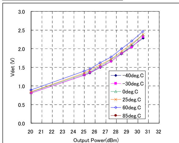
Detector Voltage vs. Output Power
