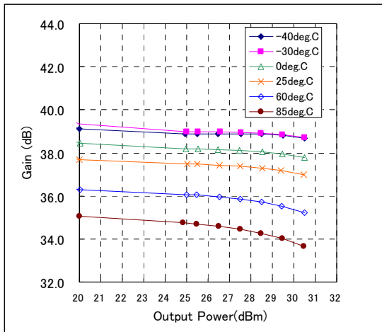
Gain vs. Output Power
