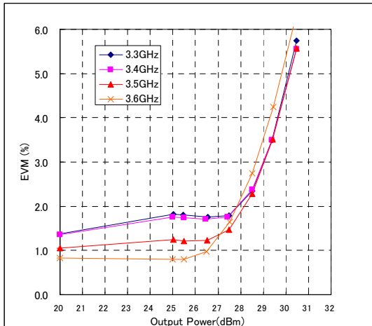
EVM vs. Output Power
