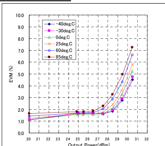
ACP Characteristics
