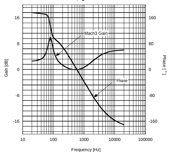
Mach3 Gain vs. Frequency
